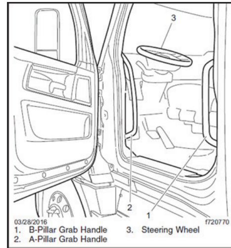
Figure 5. Driver-side entry (DTNA, 2023)
