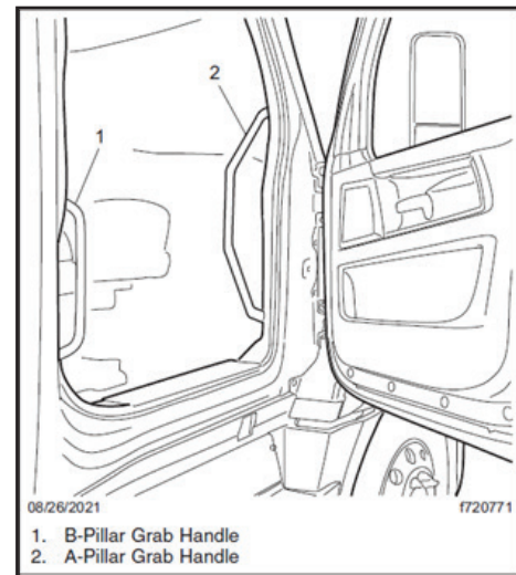
Figure 6. Passenger-side entry (DTNA, 2023)
