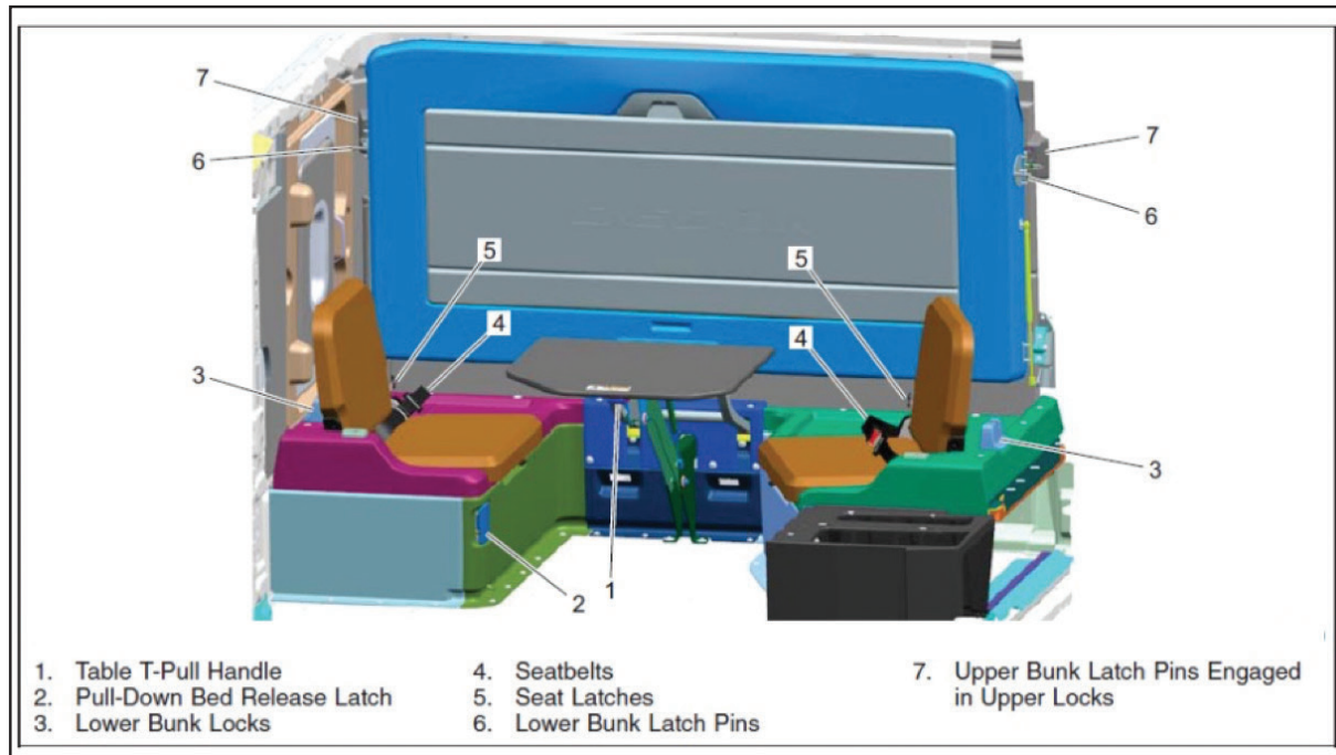
Figure 7. Rear passenger seats (DTNA, 2023)
