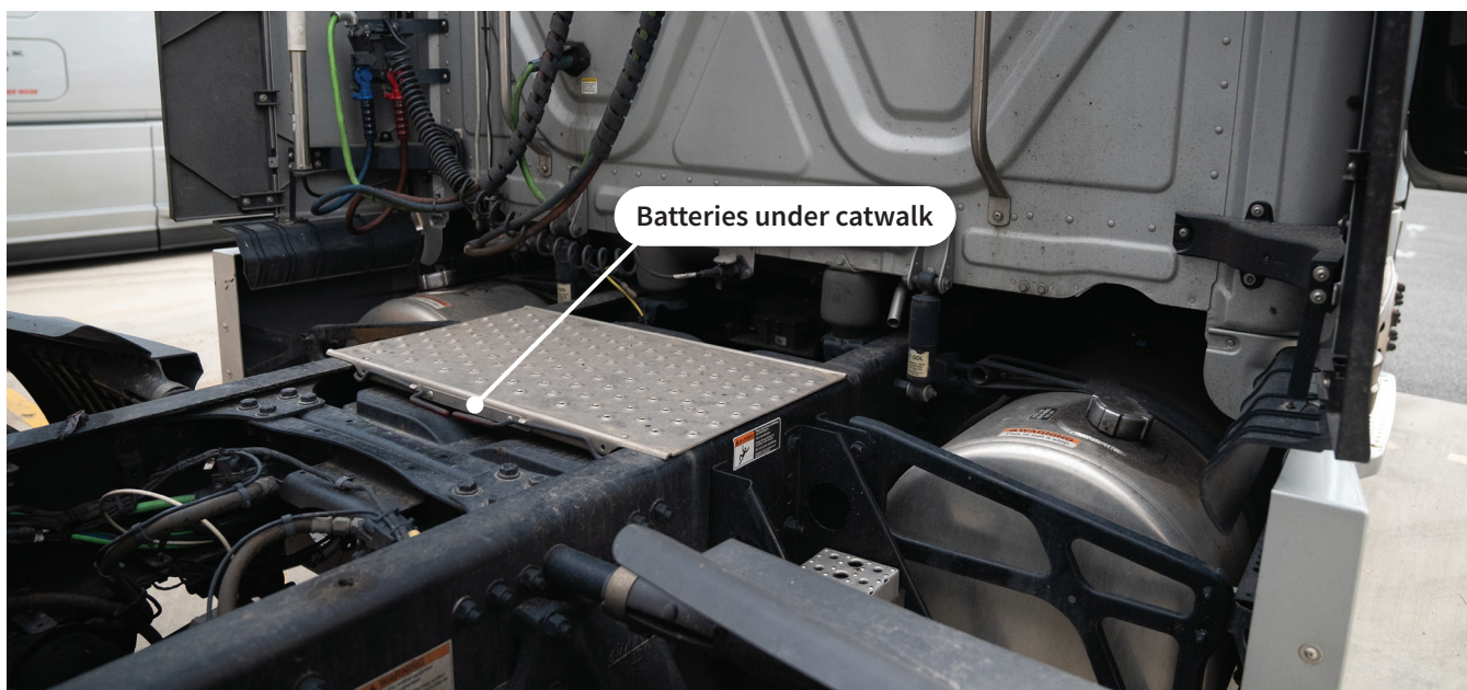
Figure 20. Location of batteries under catwalk
