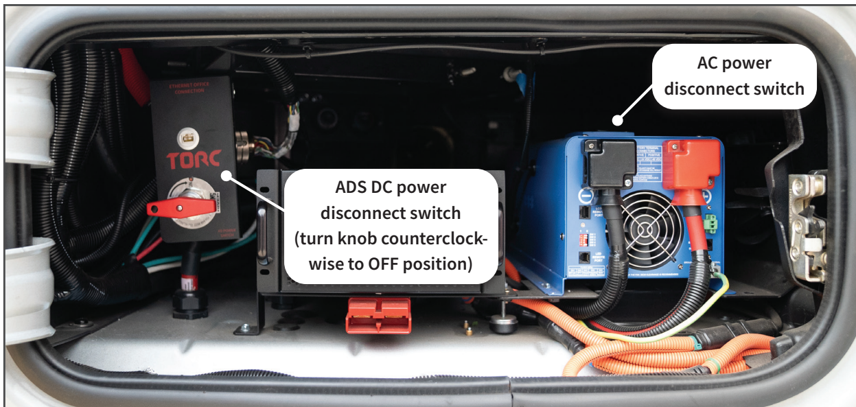
Figure 17. Location of DC and AC power disconnect switches
